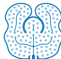
Universal Pad
